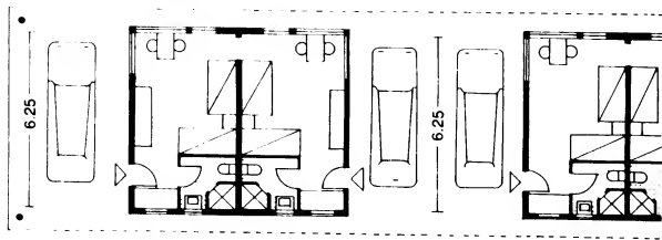
① Rooms open to one side only: furnishing options
